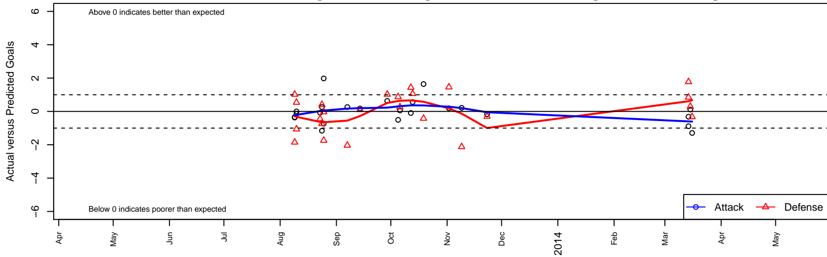
ACC Mavericks United FC B97 Dots are actual minus expected GF (blue circles) and GA (red triangles). Blue line is smoothed change in attack strength. Red is smoothed change in defense strength.
